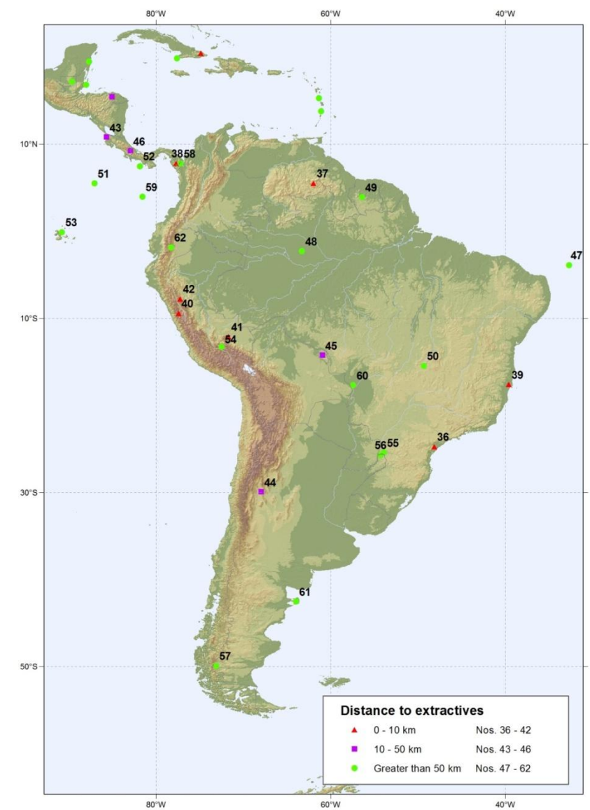
Figure 7.4: South and Central America depicting World Heritage sites categorised according to their minimum distance to active extractive operations
